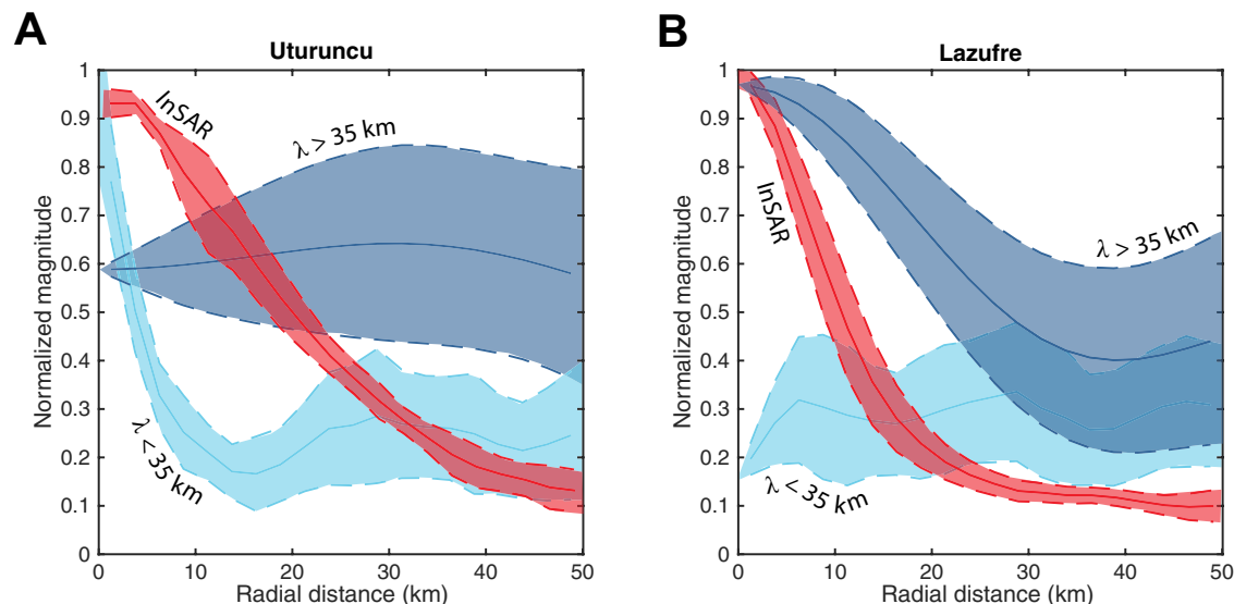
Figure 2. Normalized radial profiles of line-of-sight (LOS) velocity and the long-wavelength (>35 km) and short-wavelength (<35 km) components of topography at Uturuncu and Lazufre. LOS velocity data are from stacked interferograms created along Envisat descending track 282. Topography data comes from the global 90 m Shuttle Radar Topography Mission (SRTM) data set, and interferometric synthetic aperture radar (InSAR) data are from Henderson and Pritchard (2013). Solid lines represent the average radial value as a function of distance from the peak line LOS velocity anomaly, and dashed lines represent \pm 1\sigma . Here we use LOS velocity rather than true vertical displacement, which underestimates the true rate of vertical motion but will have little effect on the rate of tilting. Panel A shows the profiles at Uturuncu, and panel B shows the profiles for Lazufre.
